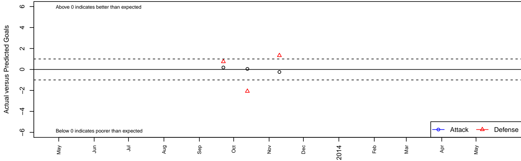
Merced United FC G99 Dots are actual minus expected GF (blue circles) and GA (red triangles). Blue line is smoothed change in attack strength. Red is smoothed change in defense strength.
